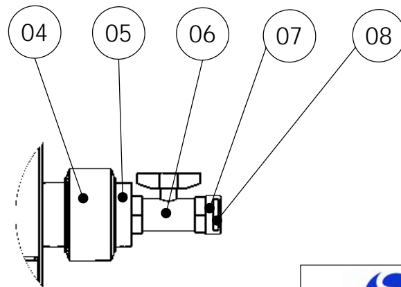
DETAIL X SCALE 1 : 5
