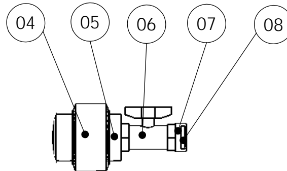
DETAIL X SCALE 1 : 5
